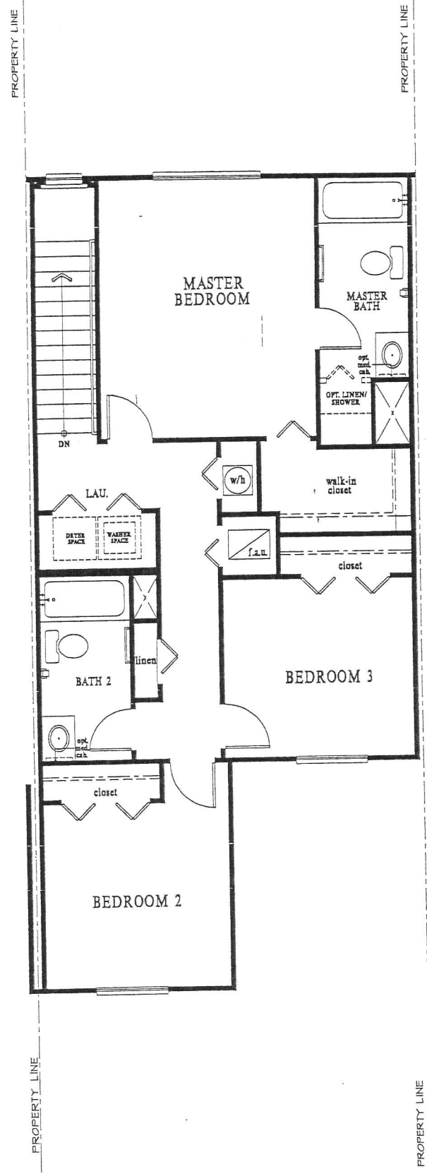
SECOND FLOOR
