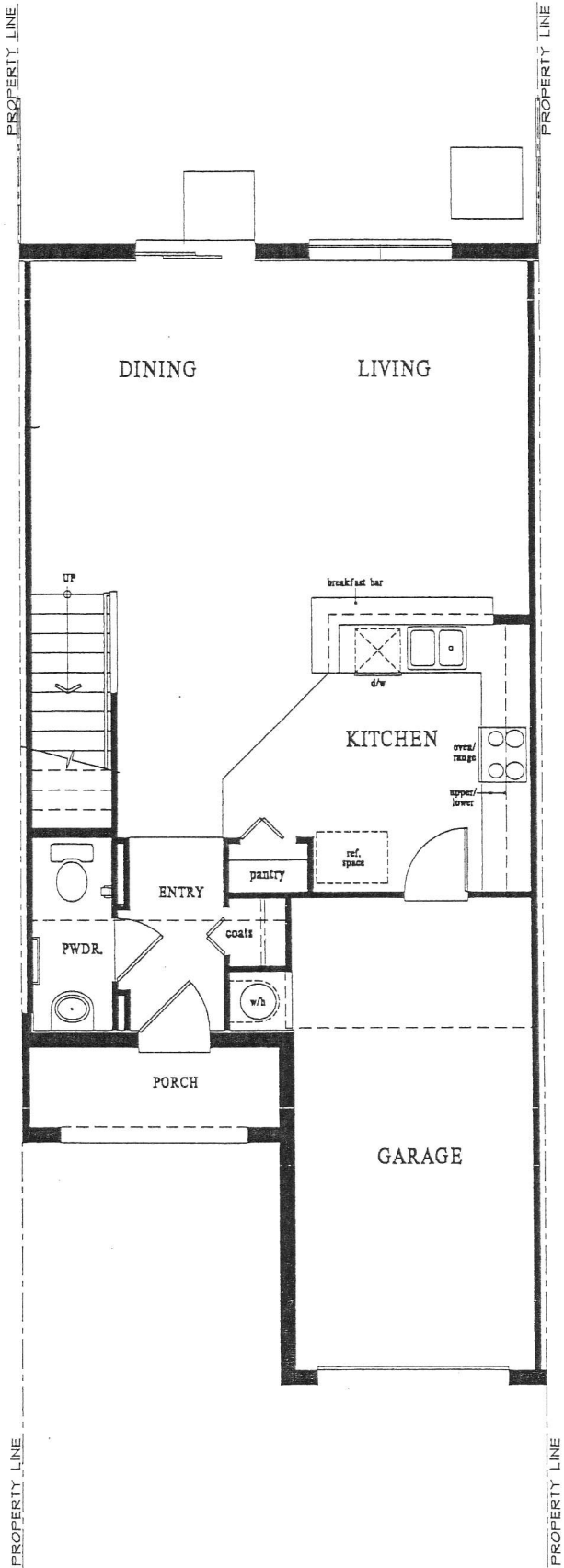
FIRST FLOOR
