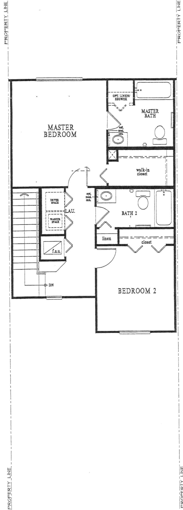
SECOND FLOOR
